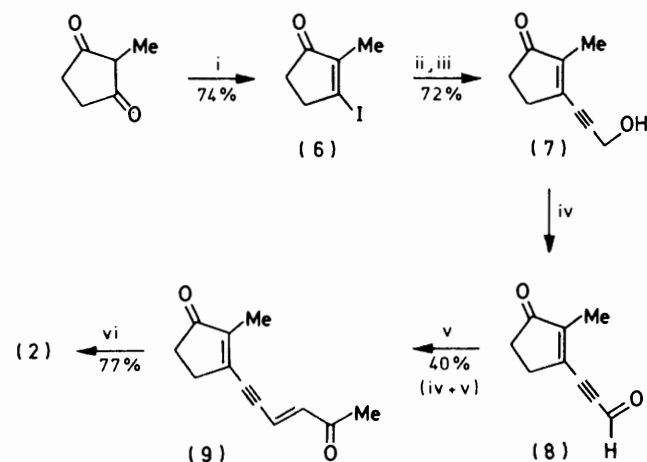
SCHEME 2 Reagents: i, \text{Ph}_3\text{PI}_2\text{-Et}_3\text{N} , 20 °C; ii, \text{CuC}\equiv\text{CCH}_2\text{-OTHP-DMF} , 125 °C; iii, \text{TsOH-MeOH} , 20 °C; iv, \text{C}_6\text{H}_5\text{NHCl}^-\text{-CrO}_3 , 20 °C; v, \text{Ph}_3\text{P}^+\text{CHCOMe} , 20 °C; vi, \text{H}_2\text{-Pd-BaSO}_4\text{-quinoline}
