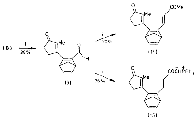
SCHEME 5 Reagents: i, cyclopentadiene, 20 °C; ii, \text{Ph}_3\text{P}^+\text{CHCOMe}^- , 56 °C; iii, \text{Ph}_3\text{P}^+\text{CHCOCH}^+\text{HPPH}_3^- (17), 20 °C
